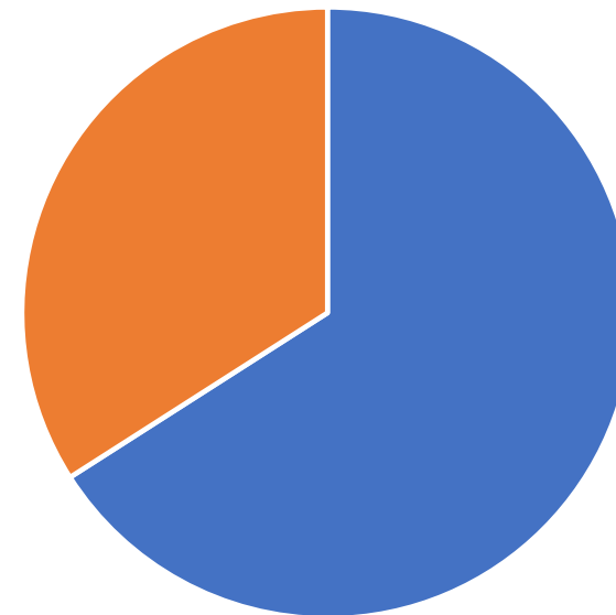
Test Coverage
